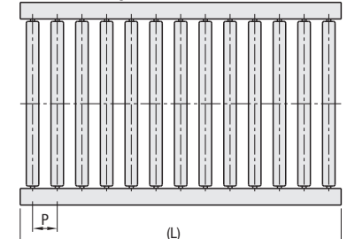
Roller Conveyor
