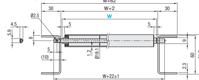
Roller Only
